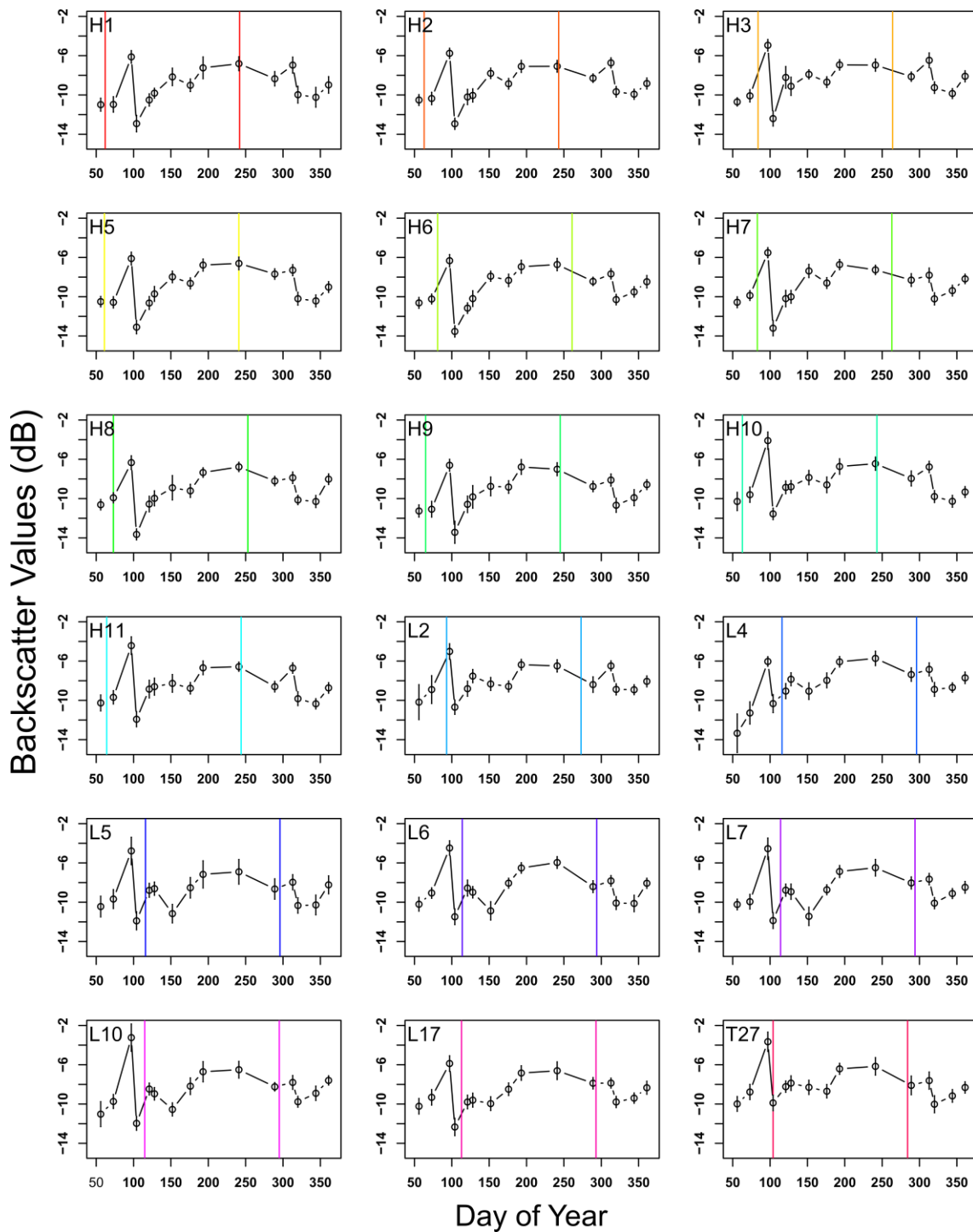
Figure 6.14: A multiplot of the Sentinel-1 (S-1) descending mode backscatter values for the 18 ADC Olingatongo maize fields analyzed for the 2015 cropping season. The vertical lines indicate the planting and harvesting days respectively.
