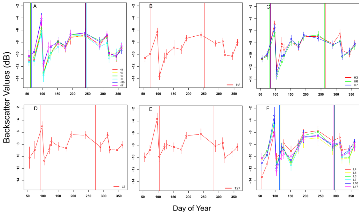
Figure 6.26: A plot of the Sentinel-1 (S-1) descending mode backscatter values for the 18 ADC Olongatongo maize fields analyzed for the 2015 cropping season grouped according to the planting dates a) 2/3-6/3 b) 14/3, c) 22/3-25/3, d) 3/4, e) 14/4, f) 23/4-26/4. The vertical lines indicate the planting and end of growth period for the maize in the fields.
