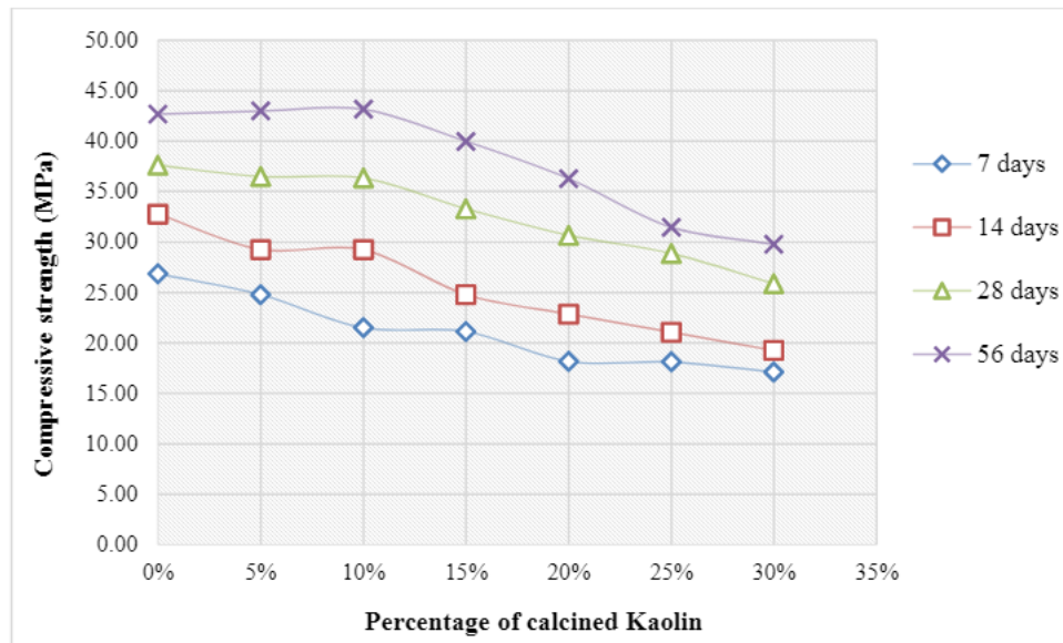
Figure 5. Compressive strength with calcined kaolin
