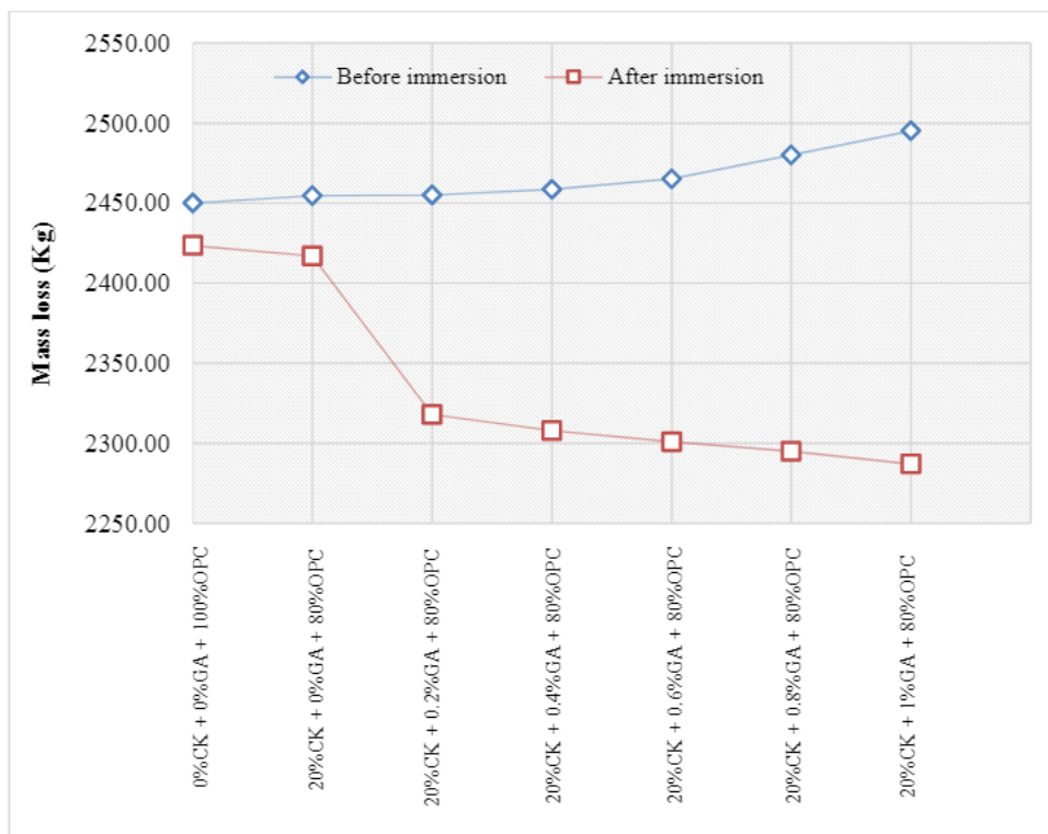
Figure 12. Mass loss at 56 days with calcined kaolin and gum Arabic
