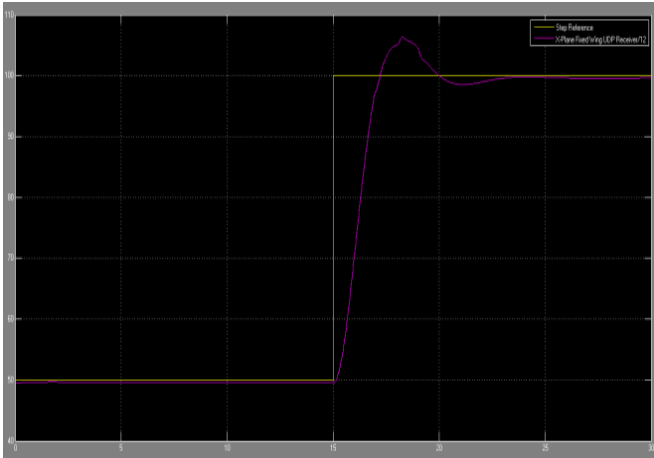
Fig. 3: PID controller response to a step heading reference
