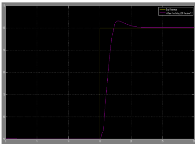
Fig. 4: RL controller response to a step heading reference
