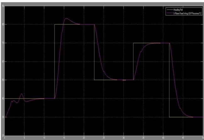
Fig. 7: RL controller response after training
