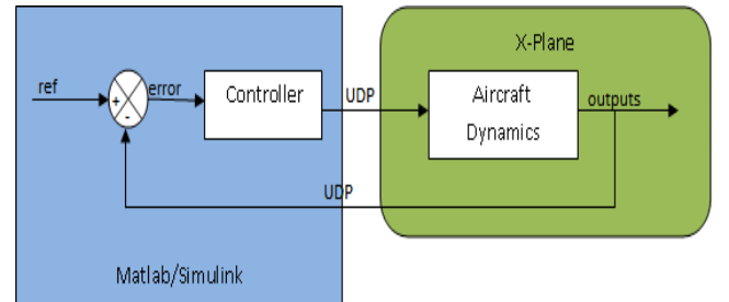
Fig. 2: Software-In-the-Loop Simulation
