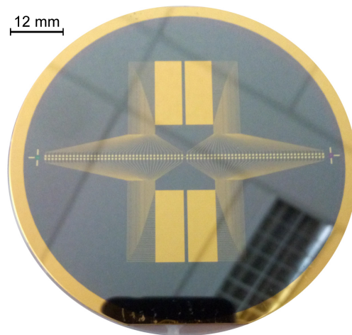
Fig. 5. electrode's array prototype.
