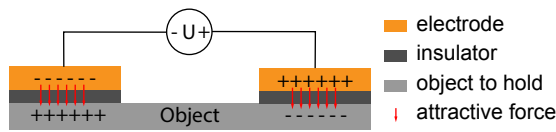
Fig. 1. Electrostatic chuck principle
