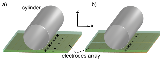
Fig. 3. FEM models. a) one column electrodes array distribution, b) two columns electrodes array distribution.
