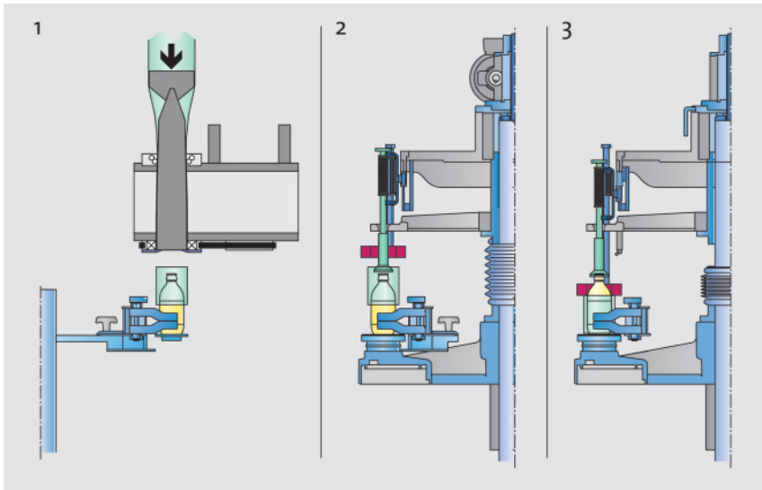
Figure 13.15 Shrink-sleeve process.
