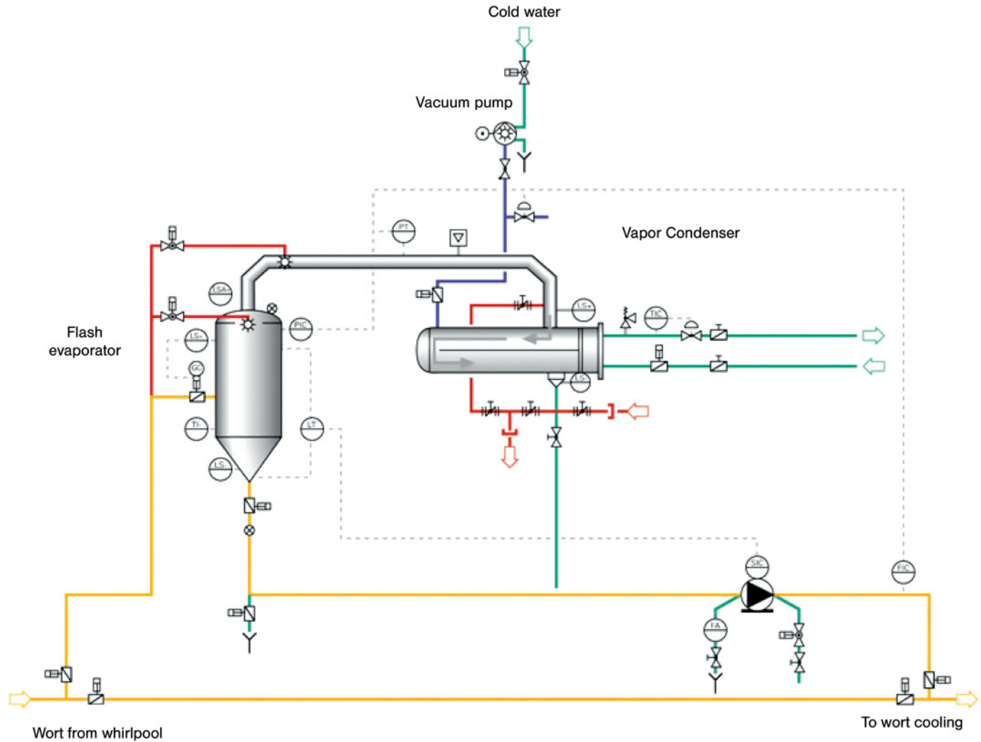
Figure 7.30 Process scheme of the vacuum evaporation system (source: A. Ziemann, Ludwigsburg, Germany).
