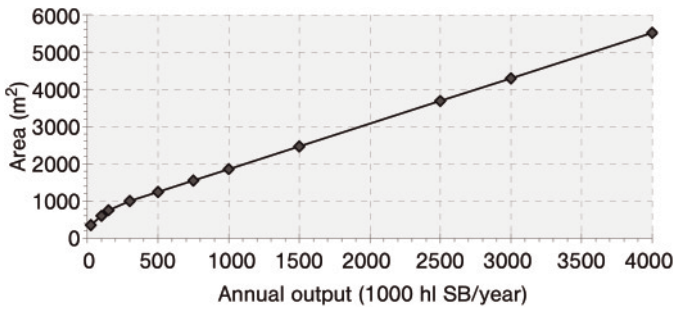
Figure 23.7 Space requirement: tanks.
