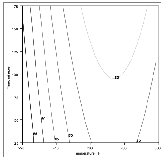
FIGURE 3.4.6.2(j) Example of quadratic response surface (adhesive peel strength in psi as a function of cure final dwell time and temperature).
