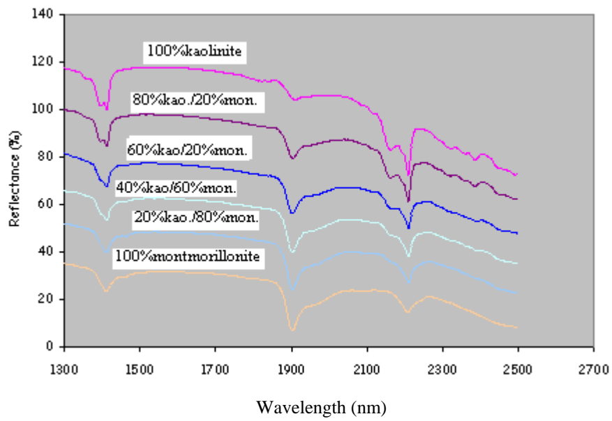
Figure 1. Changing parameters with changes in kaolinite/montmorillonite
