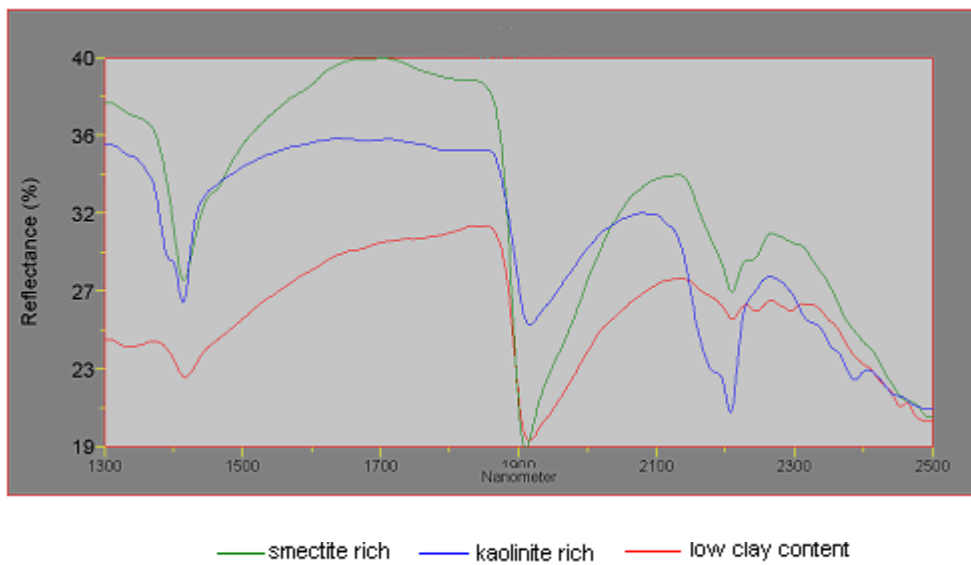
Figure 2. Spectra of some of the soil samples showing characteristic differences used in the interpretation
